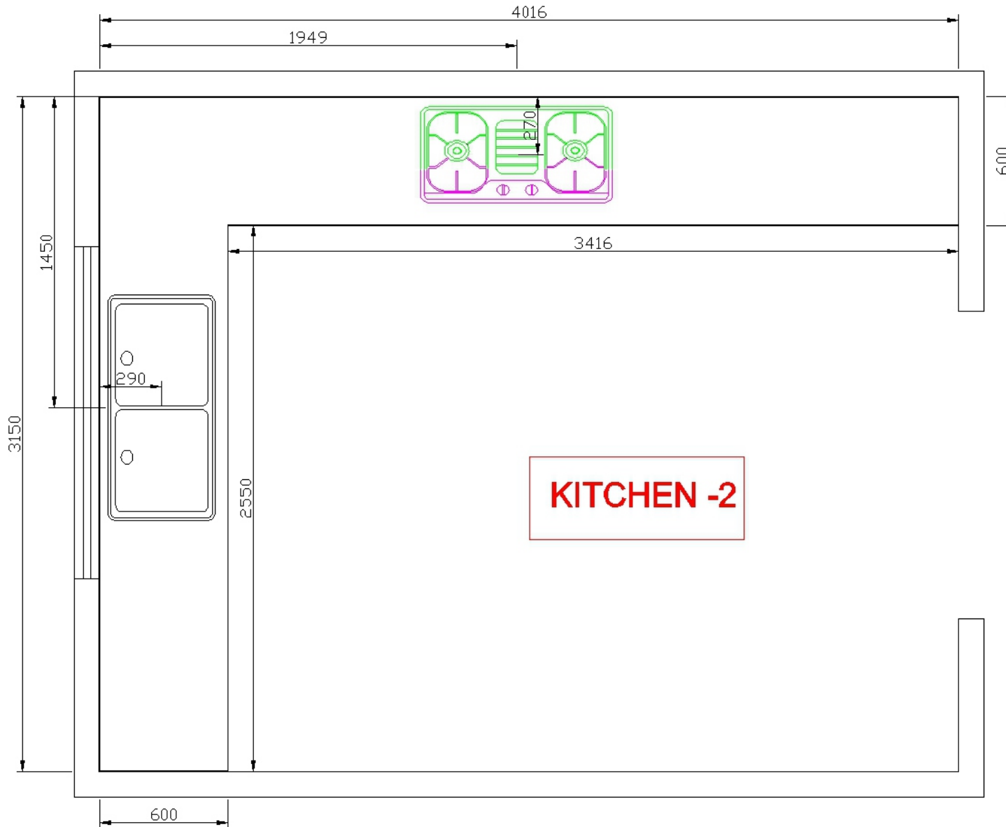
Worktop plan drawing
