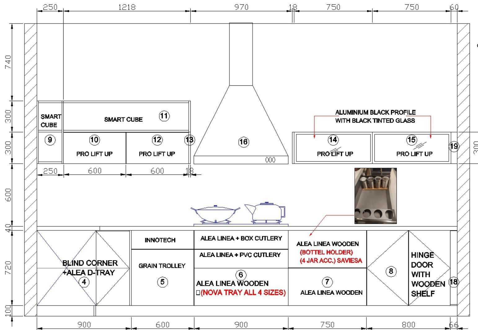
A View elevation drawing
