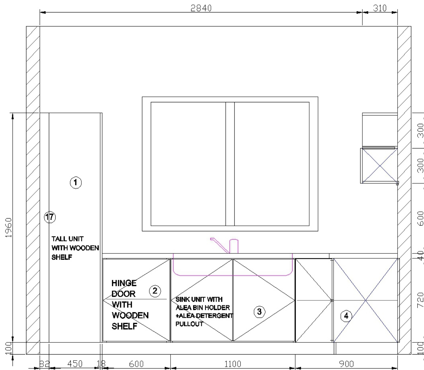
B View elevation drawing
